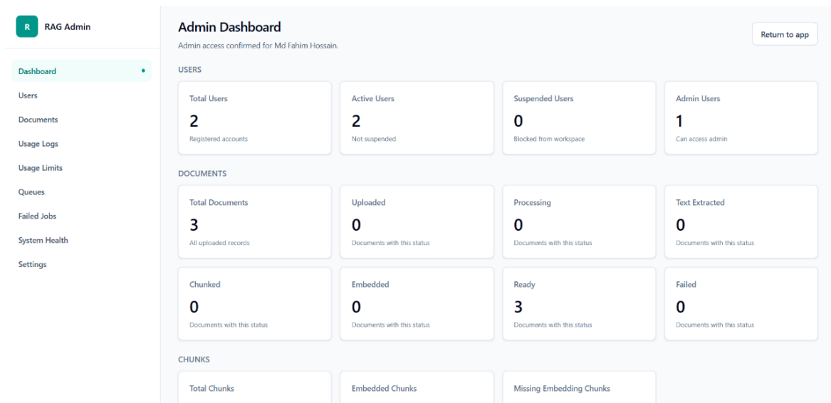
Figure 13: Administrative Dashboard
