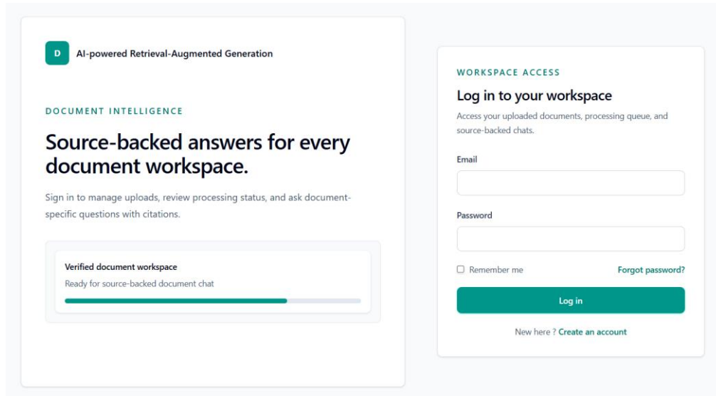
Figure 7: Login Interface
