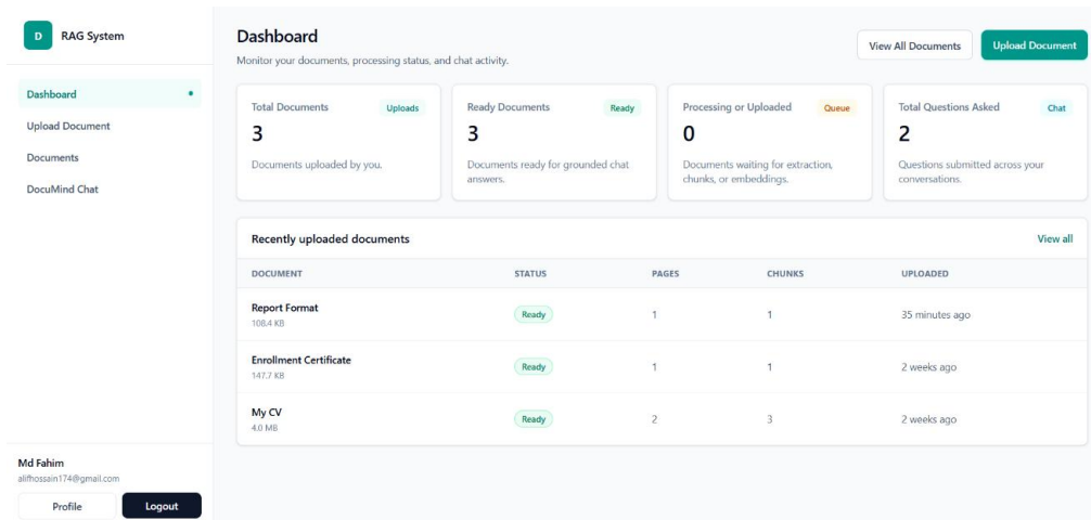
Figure 8: User Dashboard
