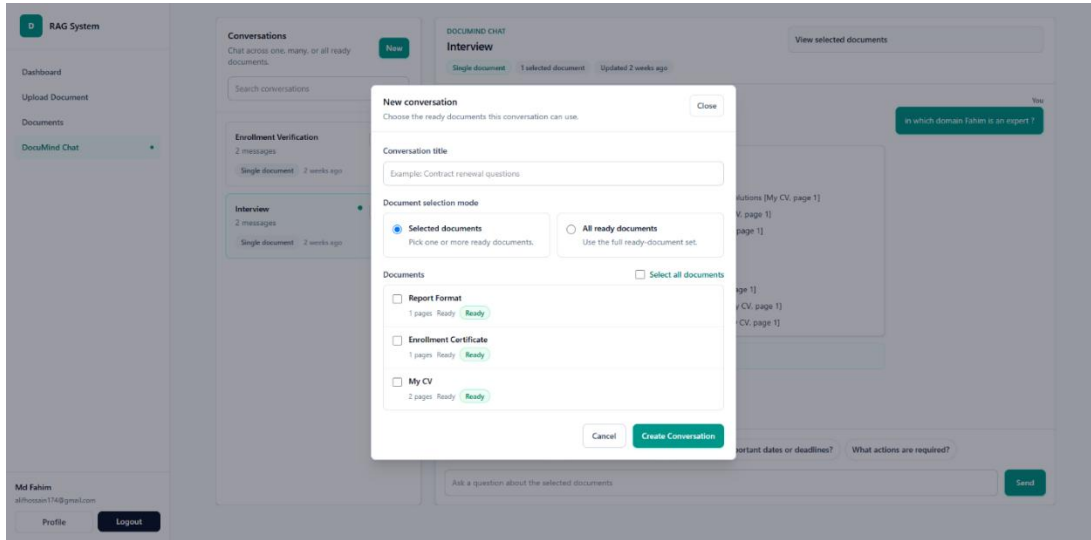
Figure 11: Conversation Interface
